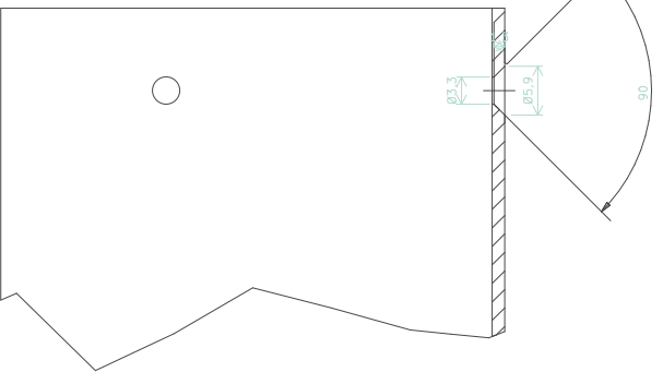
Countersink hole detail
